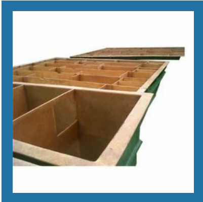
FRP Mixer Settler for Liquid Extraction System
